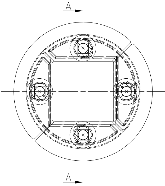
VIEW FRONT
